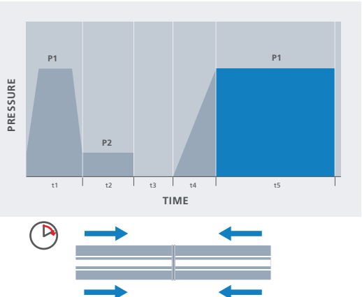
Diagram 6.13 – t5 Cooling
