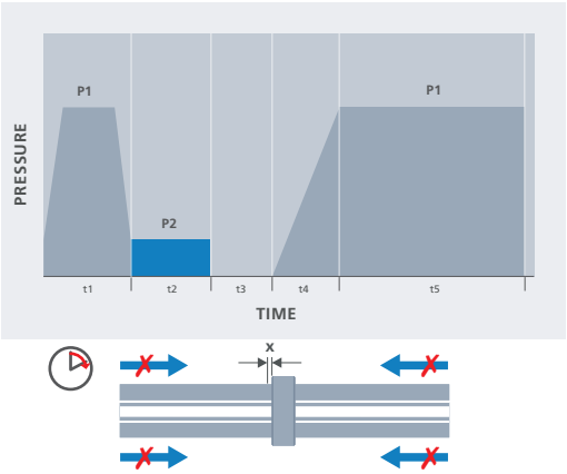
Diagram 6.10 – t2 Heating
