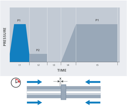
Diagram 6.09 – t1 Showing up of the welding cord
