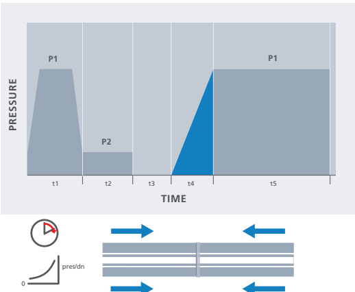
Diagram 6.12– t4 Pressure increase
